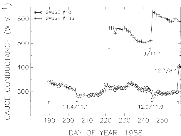
Fig. 7. Daily gauge conductance (see text) for a locally (#10) and a commercially (#186) fabricated stem flow gauge. Arrows denote placement on a plant or movement to a new plant and numbers, separated by a slash, denote the stem diameter (mm) of plant from which gauge was removed and upon which it was placed
