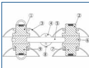
Figure 1: NR01 four-component net radiometer. SW solar radiation sensor or pyranometer (1, 9), LW Far Infra-Red radiation sensor or pyrgeometer (2, 7), radiation shield (3), leveling assembly for easy 'x' and 'y' axis adjustment (4, 5 and 8)
