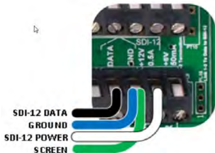
Figure 2: Sensor connection to the SDI-12 channel in the GP2 logger, using the logger's internal 12V Power channel. Colours shown are for cable type SMSC/sw-05.
