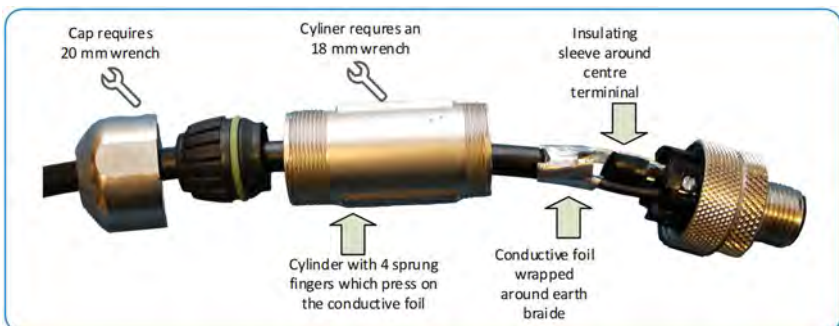
Figure 10 Exploded-view of an example of an SDI-12 sensor cable wired-up using the shielded connector.
