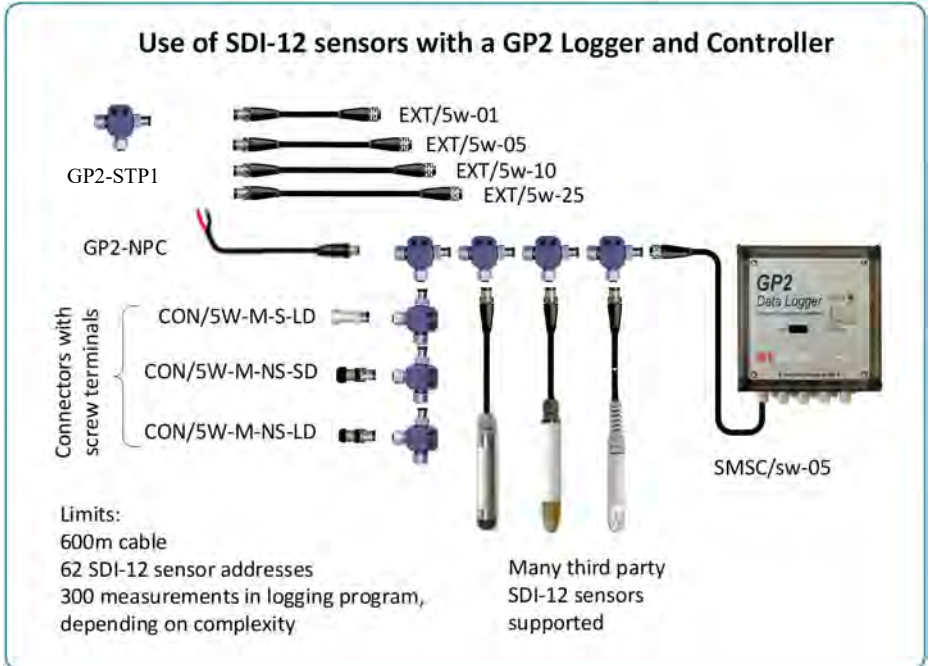
Figure 1: Wiring system used to connect SDI-12 sensors to the GP2 Logger controller, using cables with integral 5-way M12 connectors.
