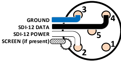
4a. Pin connections for connector type CON/5W-M-S-LD, for sensors with screened cable*
