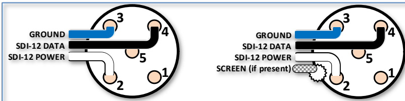
Figure 9 Wiring schemes used with the screw terminal kits, unshielded on the left, shielded on the right
