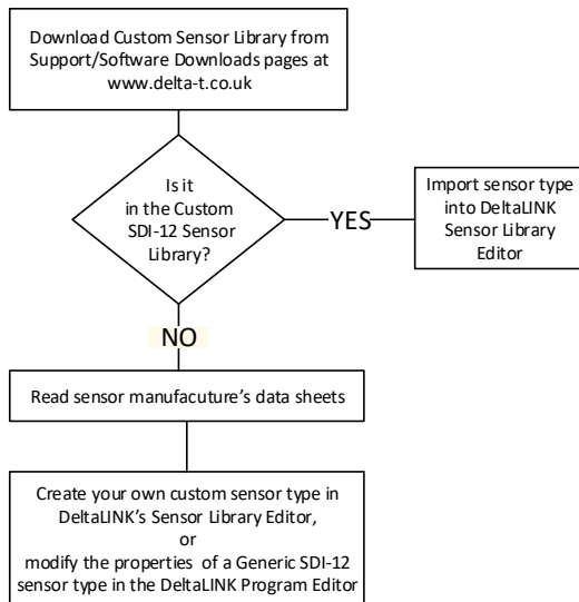
Figure 5 Decision Tree on obtaining Sensor Types for DeltaLINK for use with SDI-12 sensors from other manufacturers.
