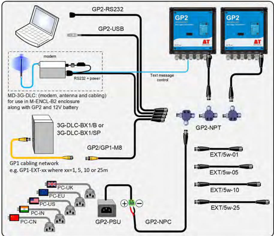
Figure A5 GP2 Network Cabling options
