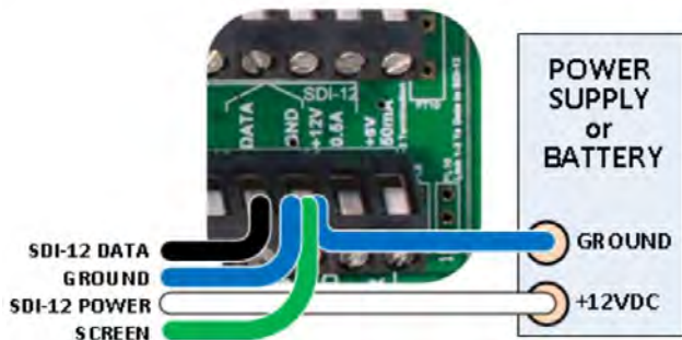
Figure 3: Sensor connection to the SDI-12 channel in GP2 logger, using an external permanent (i.e. un-switched) power supply or battery connection. Colours shown are for cable type SMSC/sw-05.
