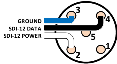
4b. Pin connections for connector types CON/5W-M-NS-(LD or SD) for sensors with unshielded cable
